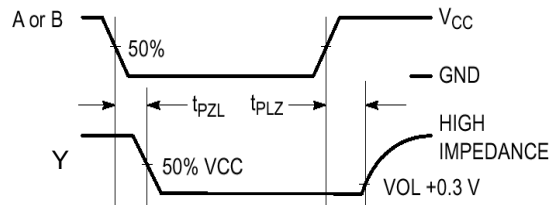
Figure 4. Switching Waveforms
