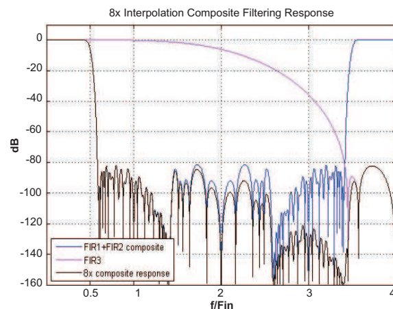
Figure 23. 8x Interpolation Composite Response
