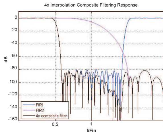
Figure 21. 4x Interpolation Composite Response
