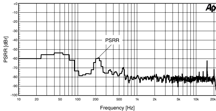
PSRR vs. Frequency
