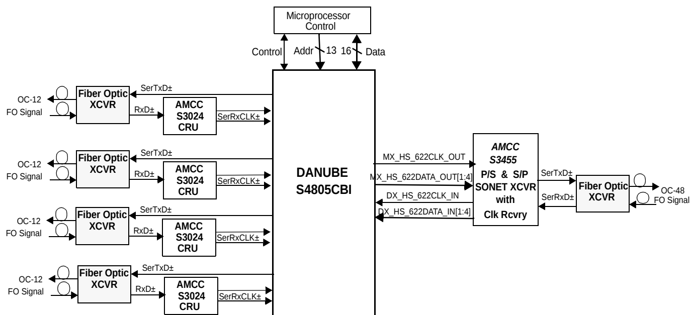
Figure 2: Typical Application
