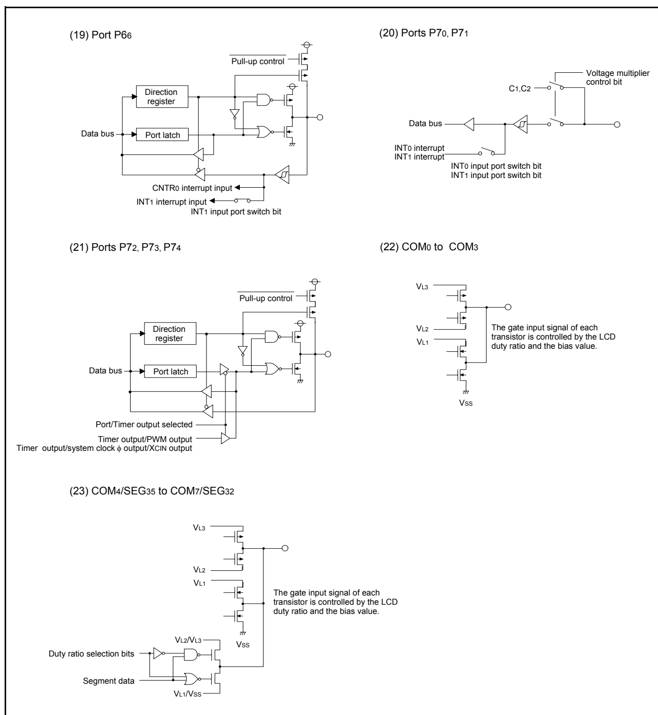
Fig. 17 Port block diagram (4)
