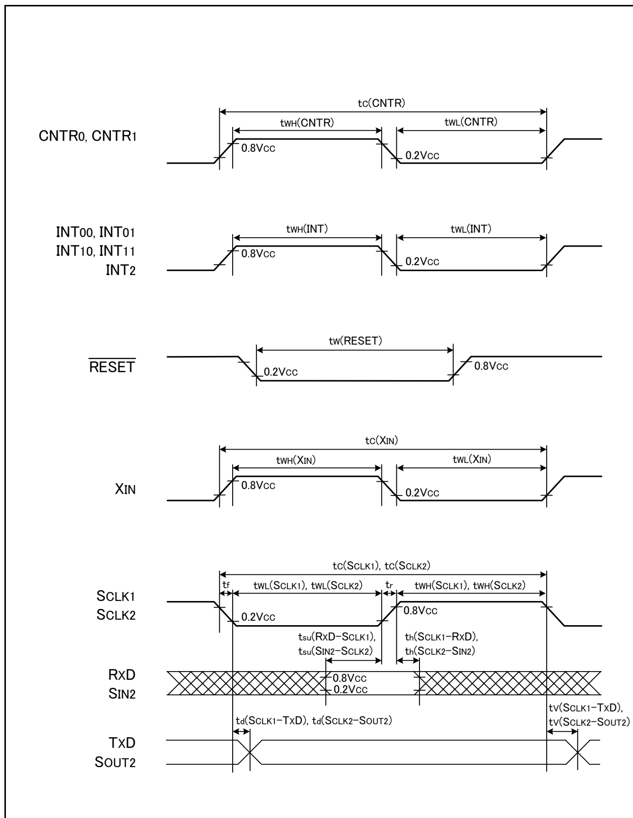
Fig 96. Timing diagram
