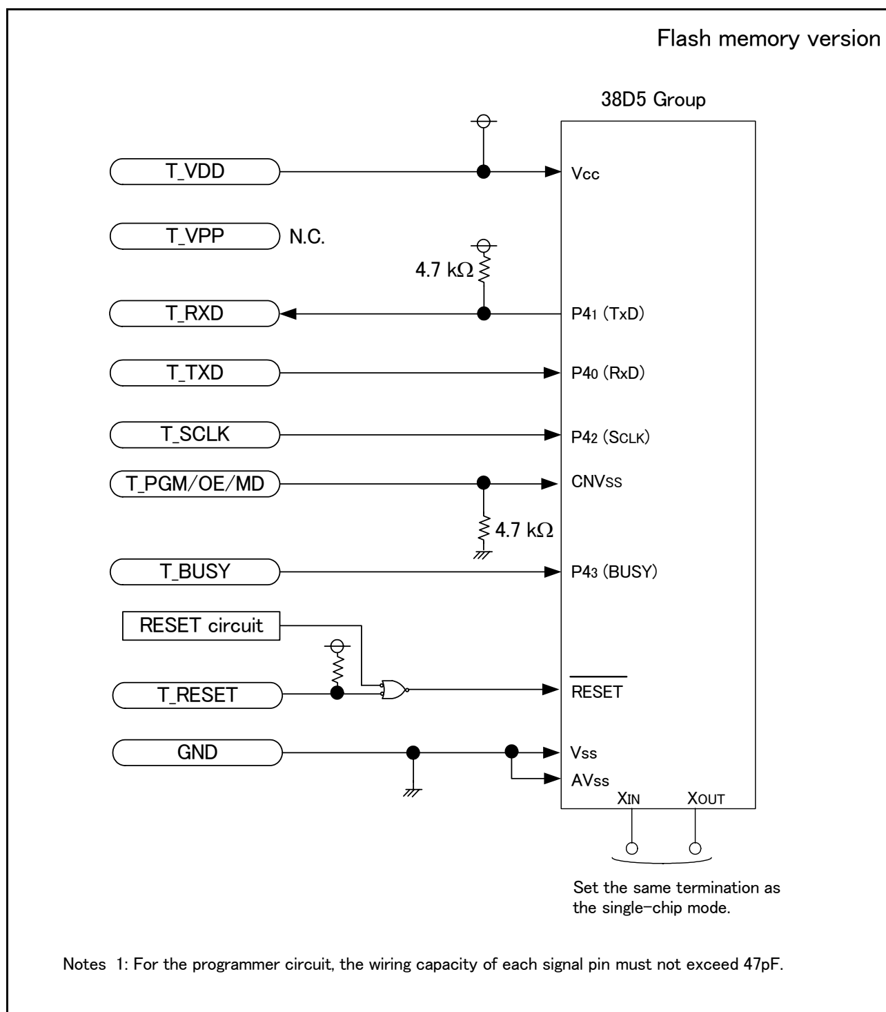
Fig 82. When using programmer (in standard serial I/O mode 1) of Suisei Electronics System Co., LTD, connection example
