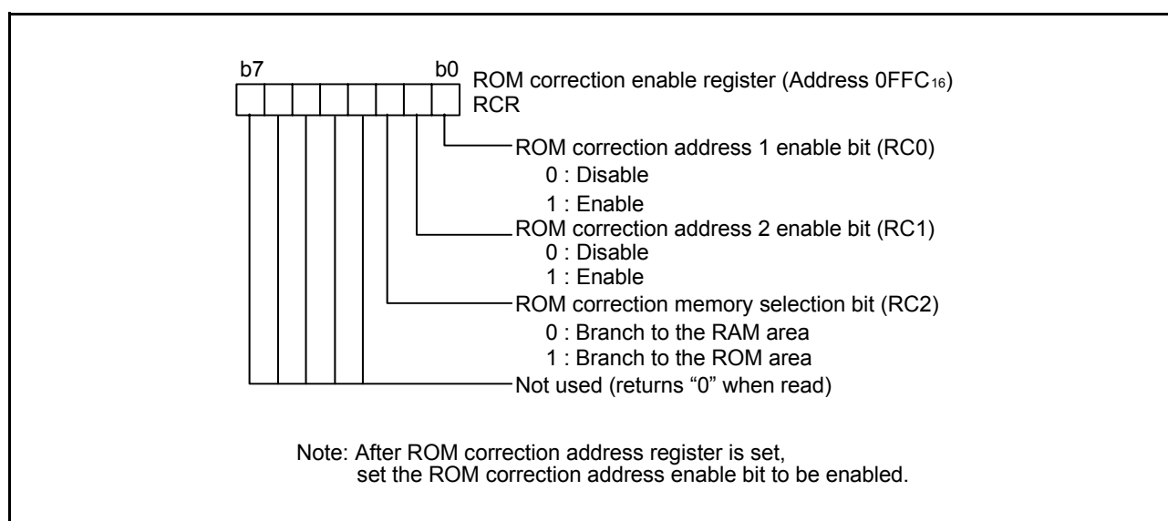
Fig. 51 Structure of ROM correction enable register
