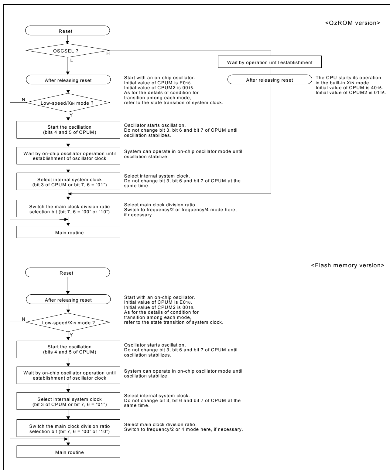
Fig. 9 Switch procedure of CPU mode register
