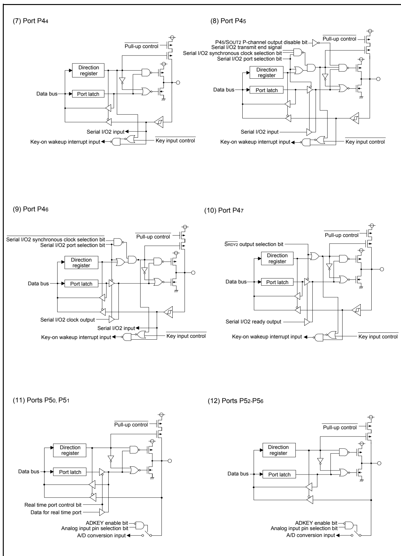
Fig. 15 Port block diagram (2)
