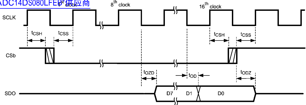
FIGURE 11. Read Timing
