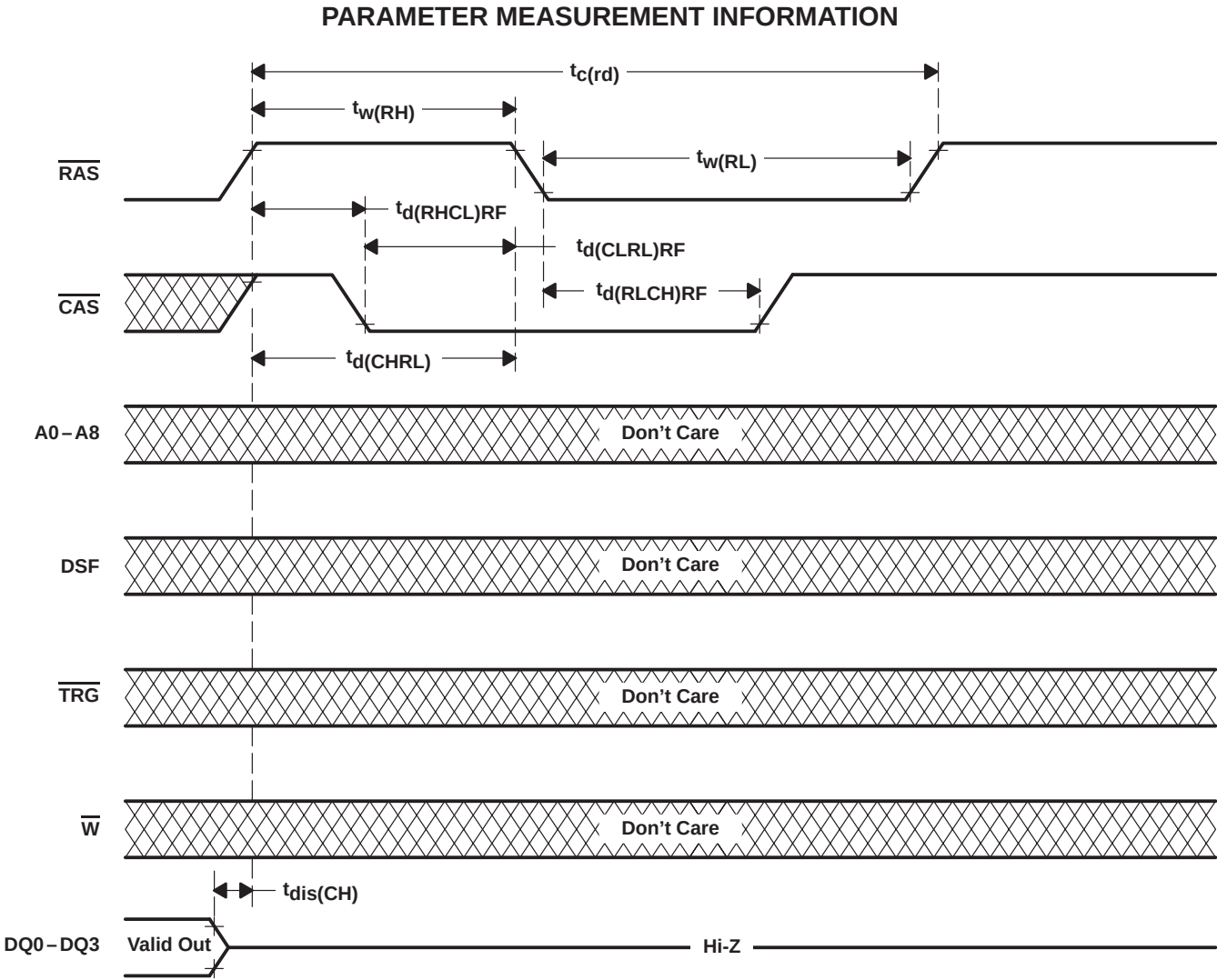
Figure 26. CBR-Refresh-Cycle Timing
