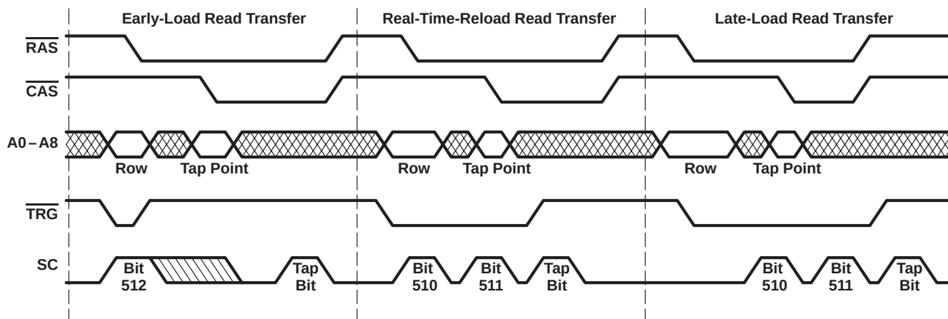
Figure 7. Normal-Read-Transfer Timings
