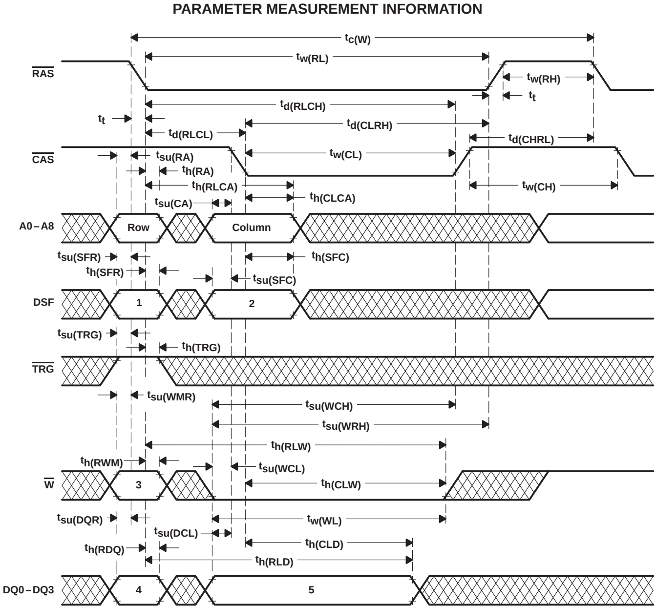
Figure 14. Early-Write-Cycle Timing
