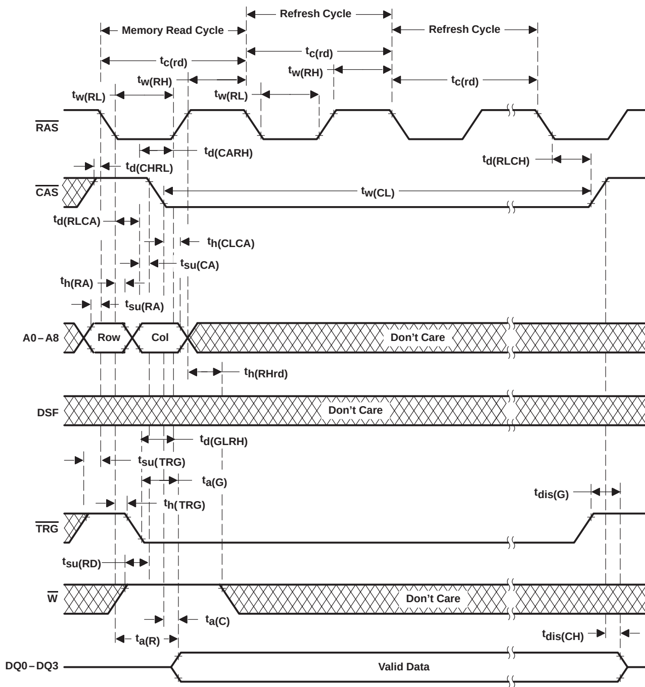
Figure 27. Hidden-Refresh-Cycle Timing
