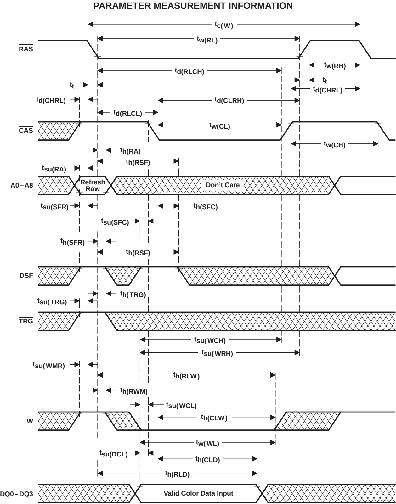
Figure 20. Load-Color-Register-Cycle Timing (Early-Write Load)
