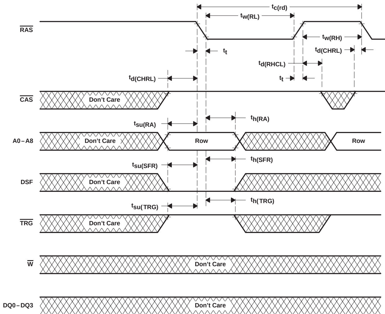
Figure 25. \overline{\text{RAS}} -Only Refresh-Cycle Timing
