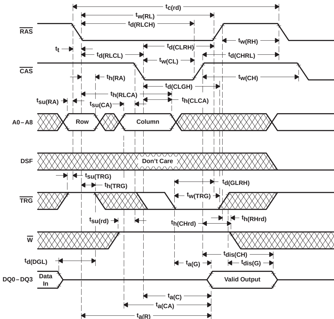
Figure 13. Read-Cycle Timing
