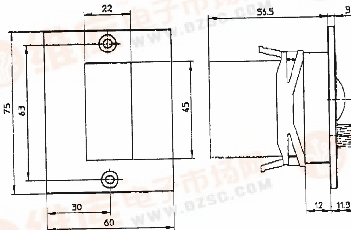
Front panel frame Type PZVT-FR
