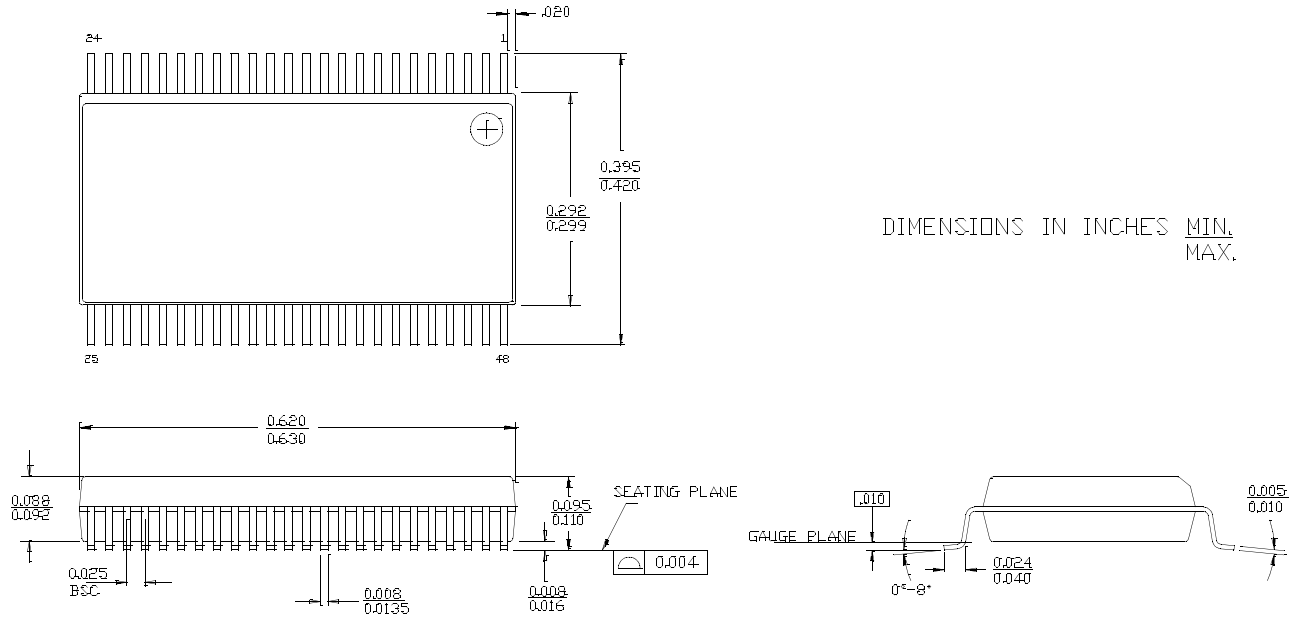
Figure 15. 48-Pin (300 mil) Shrunk Small Outline Package (51-85061)
