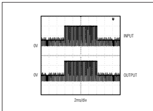
Figure 5. DirectDrive Output
