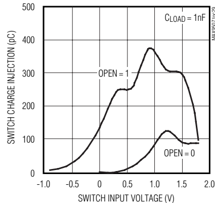
SWITCH CHARGE INJECTION vs. VOLTAGE
