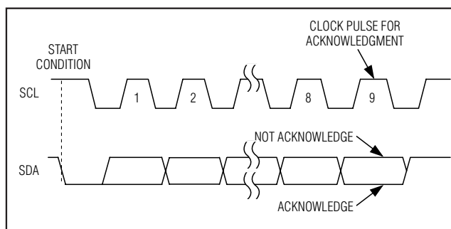
Figure 7. Acknowledge
