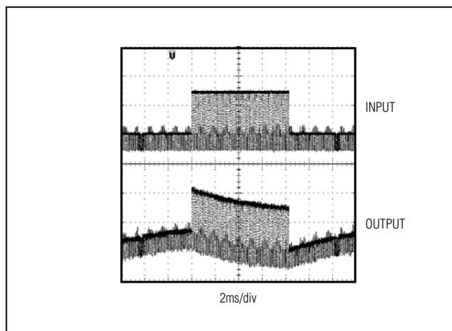
Figure 4. AC-Coupled Output
