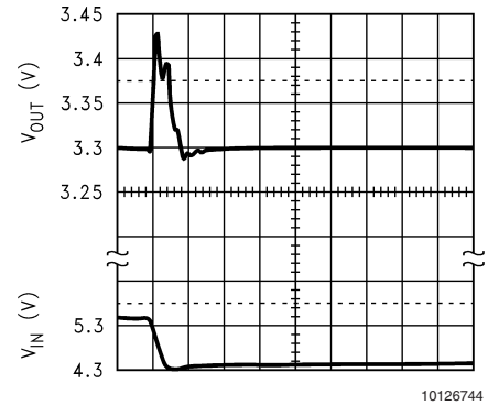
Line Transient Response ( I_{OUT} = 3.0A )
