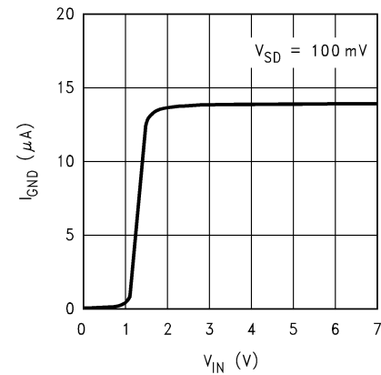
Ground Pin Current Vs Input Voltage ( V_{SD}=100\text{mV} )
