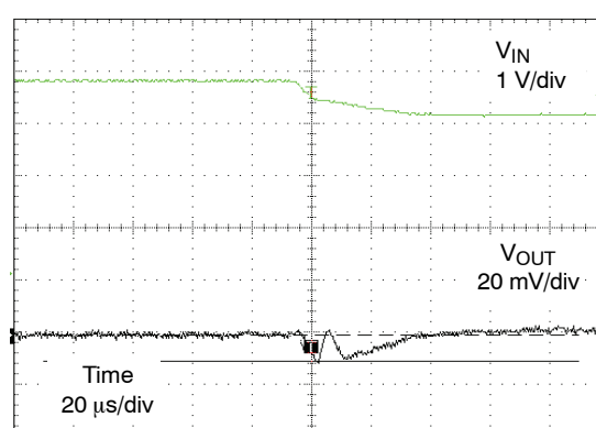
Figure 20. 3.6 V to 3.0 V Line Transient (Risetime = 50 \mu\text{s} , V_{OUT} = 1.2 \text{ V} , I_{OUT} = 100 \text{ mA} , T_A = 25^\circ\text{C} )
