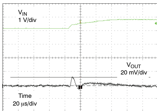
Figure 19. 3.0 V to 3.6 V Line Transient (Risetime = 50 \mu\text{s} , V_{OUT} = 1.2 \text{ V} , I_{OUT} = 100 \text{ mA} , T_A = 25^\circ\text{C} )
