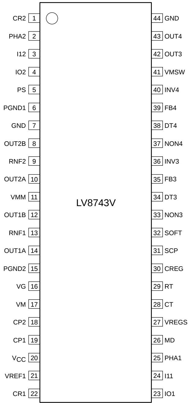
Top view
