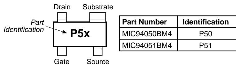
SOT-143 Package (M4)
