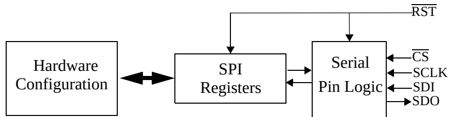
Figure 15. SPI Interface Block Diagram
