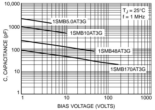
Figure 5. Typical Junction Capacitance vs. Bias Voltage
