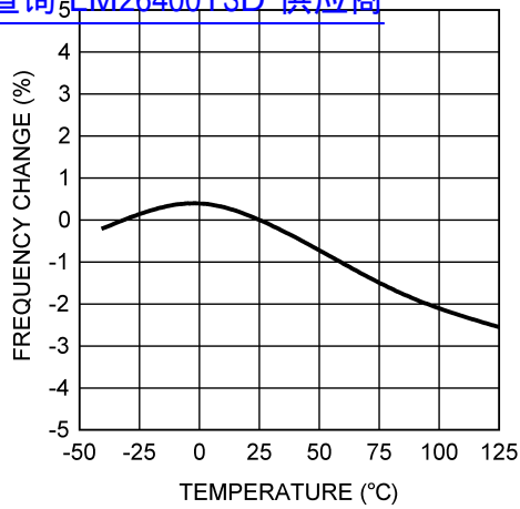
Switching Frequency vs. Temperature 查询"LM26400YSD"供应商
