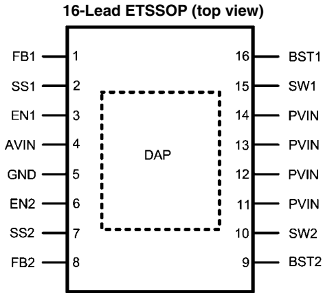
NS Package Drawing MXA16A
