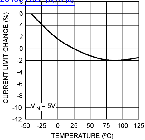
Switch Current Limit vs. Temperature 查询"LM26400YSD"供应商
