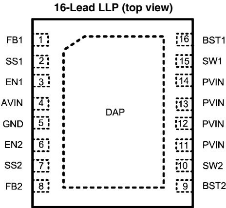
NS Package Drawing SDA16A
