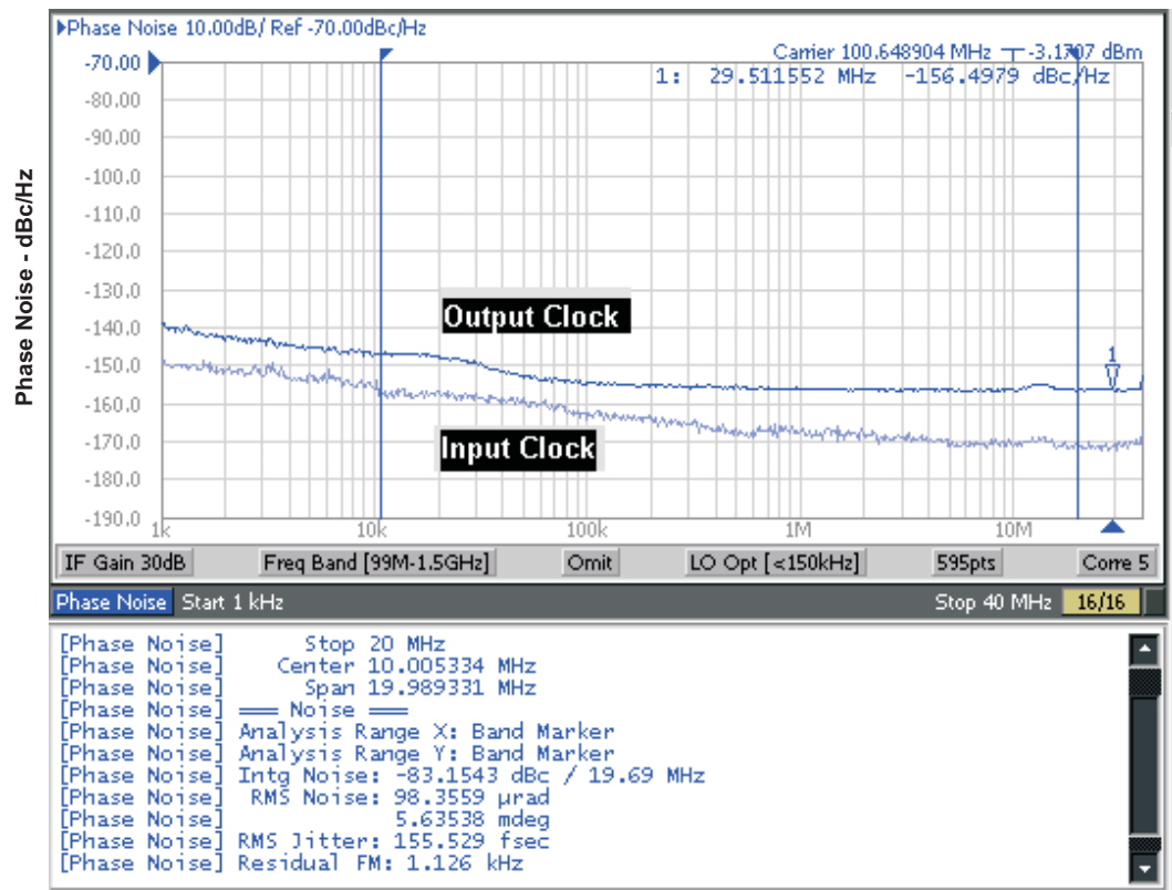
Input clock RMS jitter is 32 fs from 10 kHz to 20 MHz and additive RMS jitter is 152 fs Figure 3. 100 MHz Input and Output Phase Noise Plot
