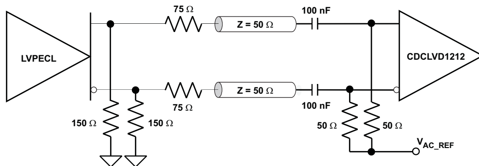
Figure 17. LVPECL Clock Driver Connected to CDCLVD1212 Input
