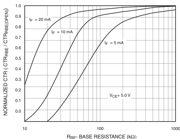
Fig. 8 CTR vs. RBE (Unsaturated) (White Package)
