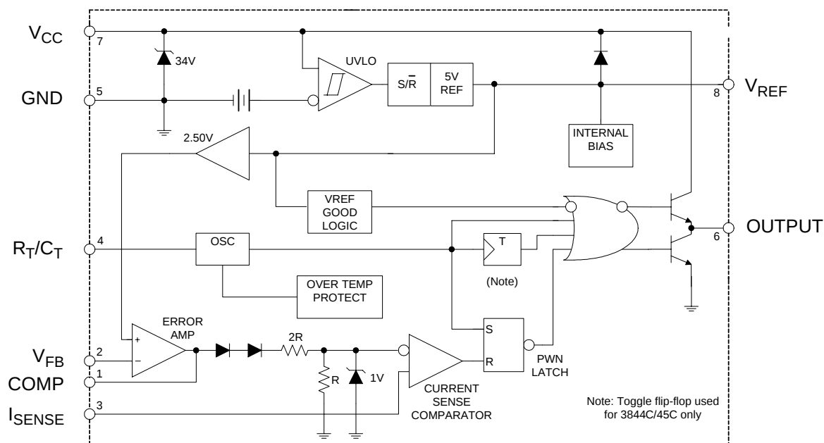
Figure 3. Functional Block Diagram of AP3842C/3C/4C/5C
