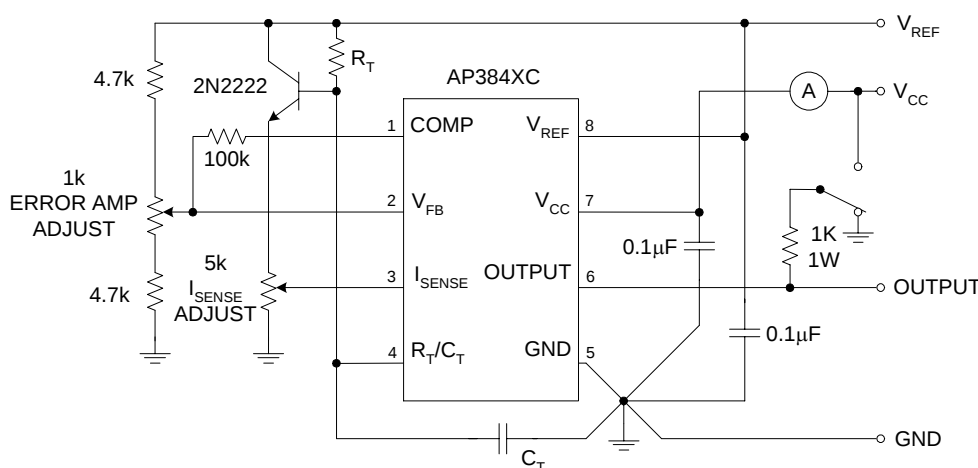
Figure 4. Basic Test Circuit
