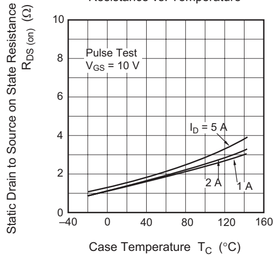
查询"2SK1773-5"供应商 Static Drain to Source on State Resistance vs. Temperature
