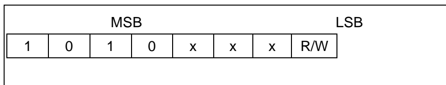
Figure 7 · Device Address
