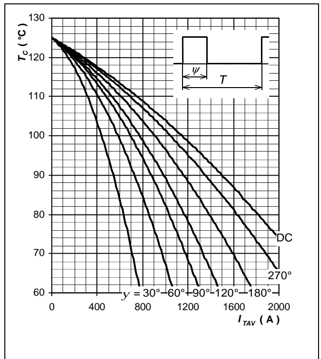
Fig. 9 Max. case temperature vs. average forward current, square waveform, f = 50 Hz, T = 1/f
