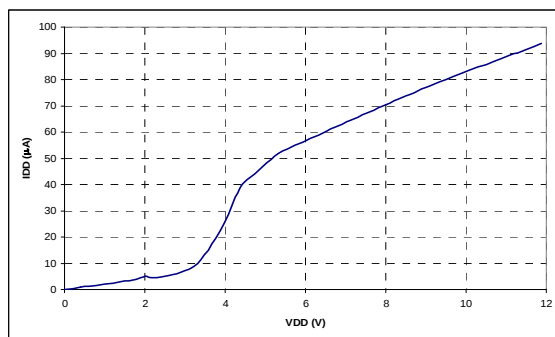
Figure 4: I_{DD} Quiescent ( I_{DD\_QST} ) vs. V_{DD}
