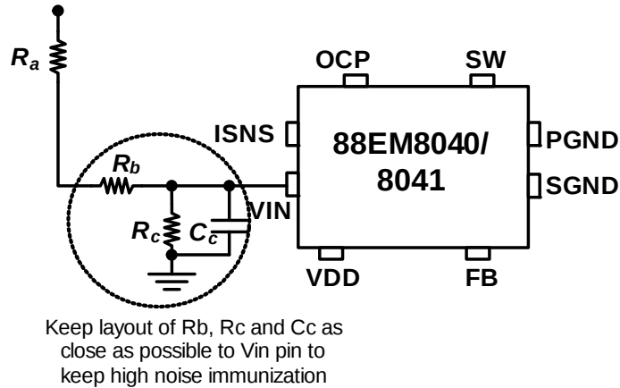
Figure 19: Input Voltage Resistor Divider Layout Guidelines
