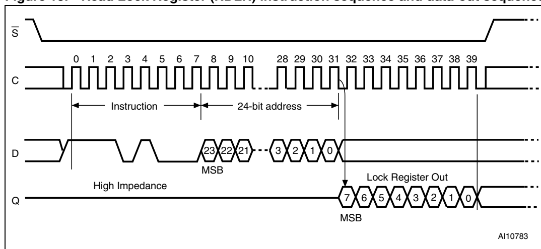
Figure 15. Read Lock Register (RDLR) instruction sequence and data-out sequence
