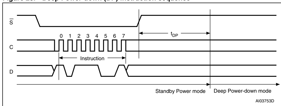
Figure 23. Deep Power-down (DP) instruction sequence
