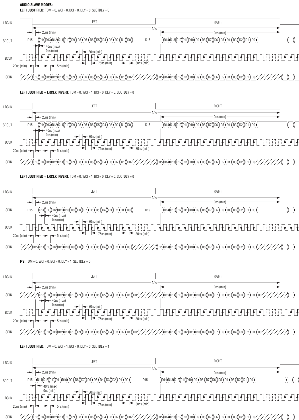
Figure 2. Digital Audio Interface Audio Slave Mode
