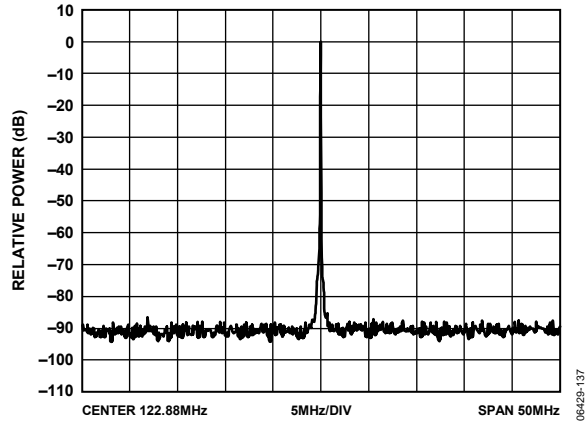
Figure 12. PFD/CP Spurs; 122.88 MHz; PFD = 15.36 MHz; LBW = 190 kHz; I_{CP} = 4.2 mA; f_{VCO} = 2.7 GHz
