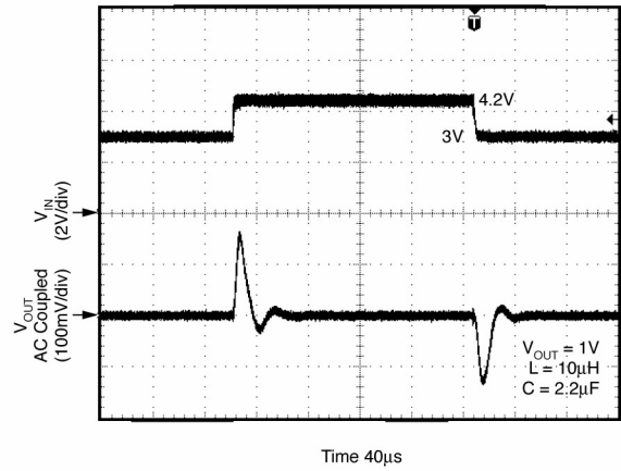
Line Transient
