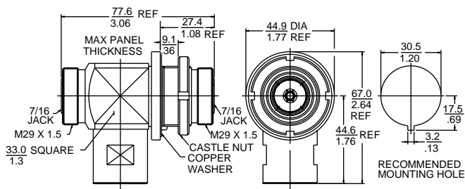
7-16 Jack to 7-16 Bulkhead Jack Adapter
