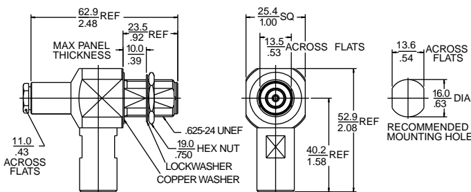
Type N Clamp Bulkhead Jack
