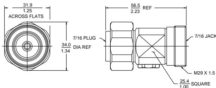
7-16 Plug to 7-16 Jack Adapter
