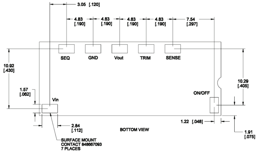
Bottom View
