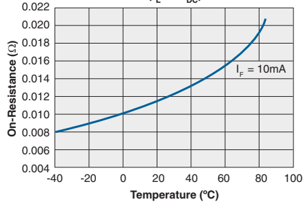
CPC1709 Typical On-Resistance vs. Temperature ( I_L = 1A_{DC} )
