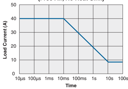
CPC1709 Energy Rating Curve (Free Air, No Heat Sink)
