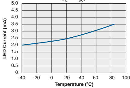
CPC1709 Typical I_F for Switch Operation vs. Temperature ( I_L = 1A_{DC} )
