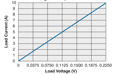
CPC1709 Typical Load Current vs. Load Voltage ( T_A = 25^\circ\text{C} , I_F = 10\text{mA} )
