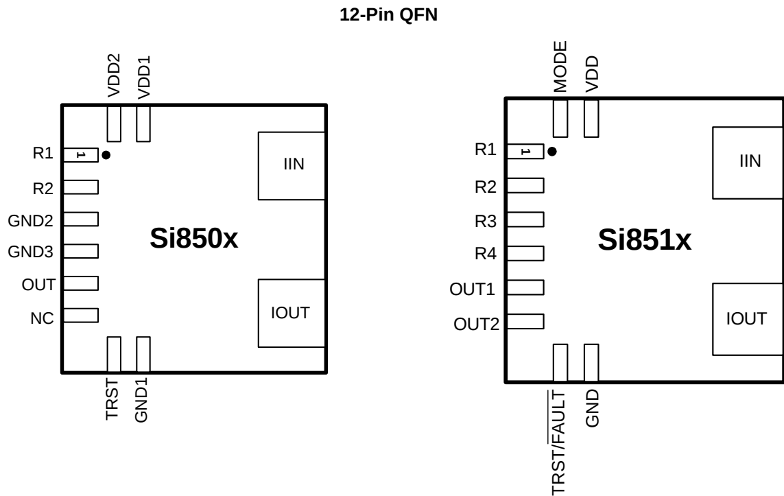
Figure 17. Example Pin Configurations
