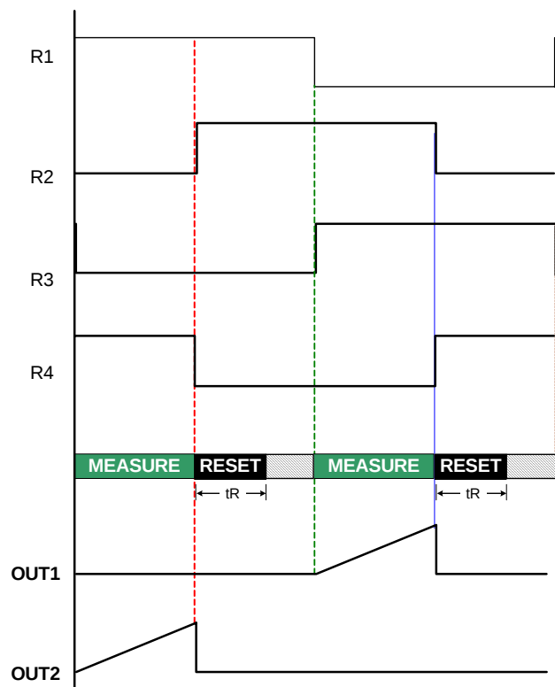
Figure 10. Full-Bridge Timing Example B
