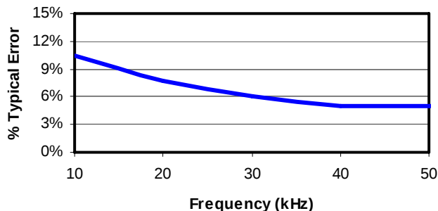
Figure 5. Full-Scale Error vs. Frequency
