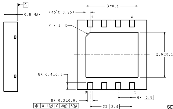
LLP Package NS Package Number SDC08A
