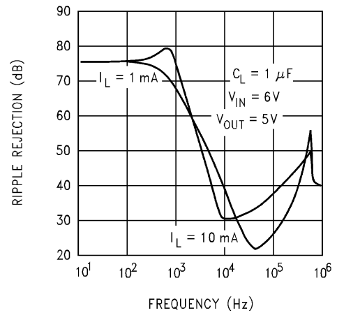
Ripple Rejection
