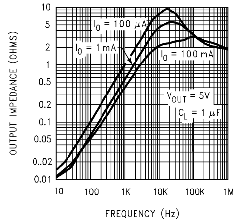
Output Impedance
