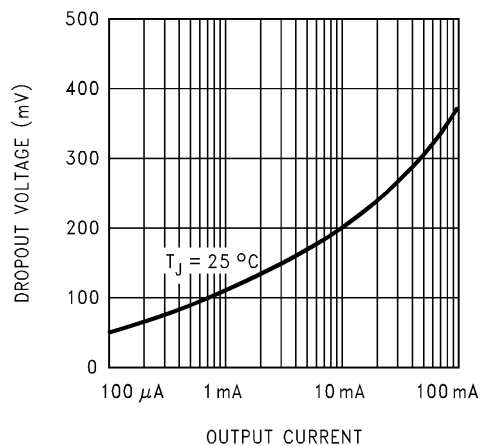
Dropout Voltage
