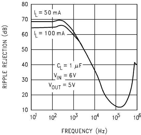
Ripple Rejection
