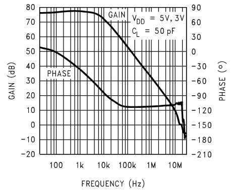
Amplifier Open Loop vs Frequency Response
