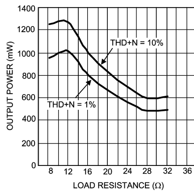
Output Power vs Load Resistance V_{DD} = 4.2V
