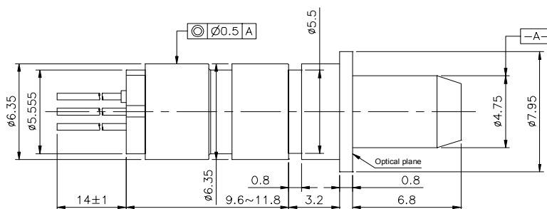
SC TOSA C-XXXXX-DFB-TX-SSCXX
