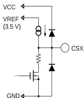
<<Soft-start block>>
