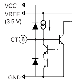
<<Triangular wave oscillator block (CT) >>
