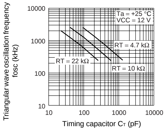
Triangular Wave Oscillation Frequency vs. Timing Capacitor
