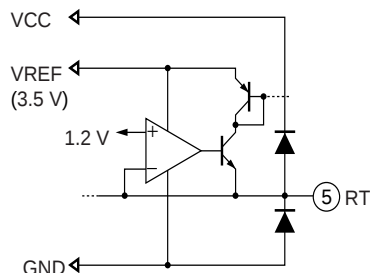
<<Triangular wave oscillator block (RT) >>
