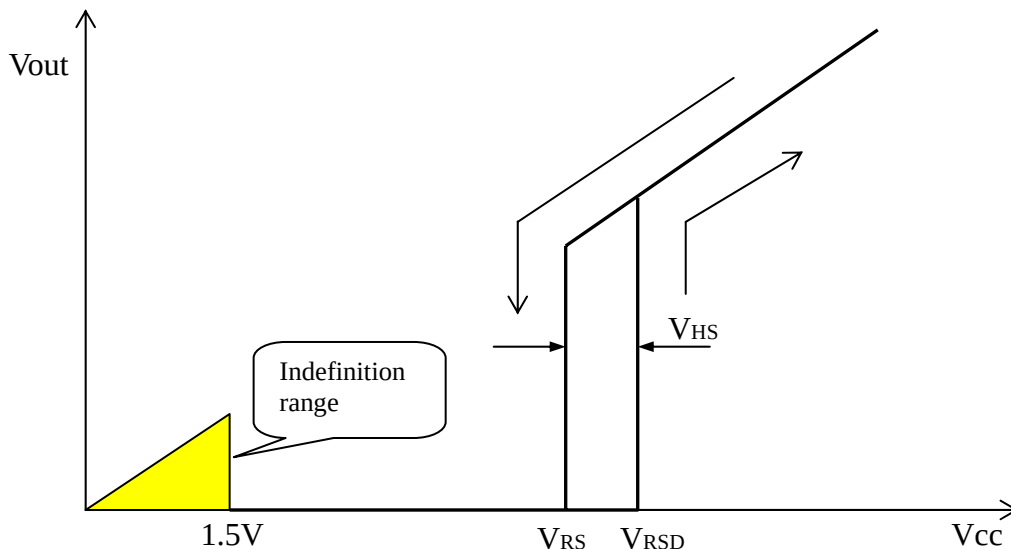
Fig-2 : Hysteresis Chart
