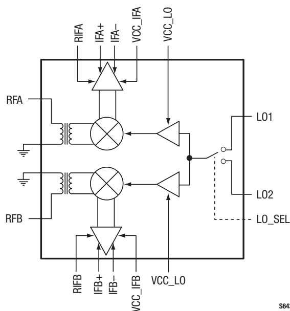
Figure 1. SKY73022-11 Block Diagram
