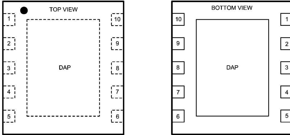
10-Pin LLP (3mm × 3mm × 0.8mm)
