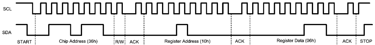
FIGURE 5. Write Sequence to the LM3509
