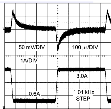
Transient Response 4V IN 20V OUT 0.6A STEP 查询"LMZ14203EXT"供应信息
