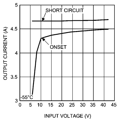
Current Limit 3.3V OUT @ -55°C
