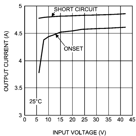
Current Limit 3.3V OUT @ 25°C
