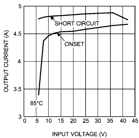
Current Limit 3.3V OUT @ 85°C
