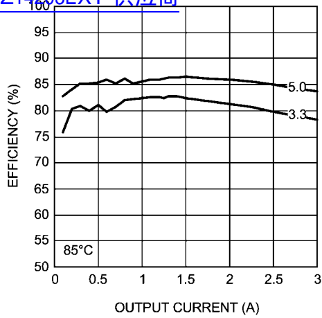
Efficiency 36V input @ 85°C 查询"LMZ14203EXT"供应商
