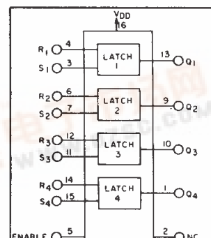
CD4044B FUNCTIONAL DIAGRAM
