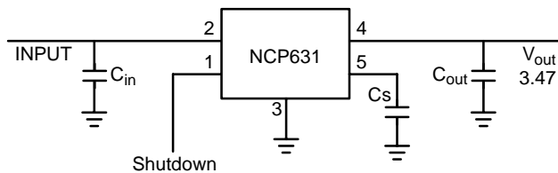
Figure 1. Typical Application Circuit
