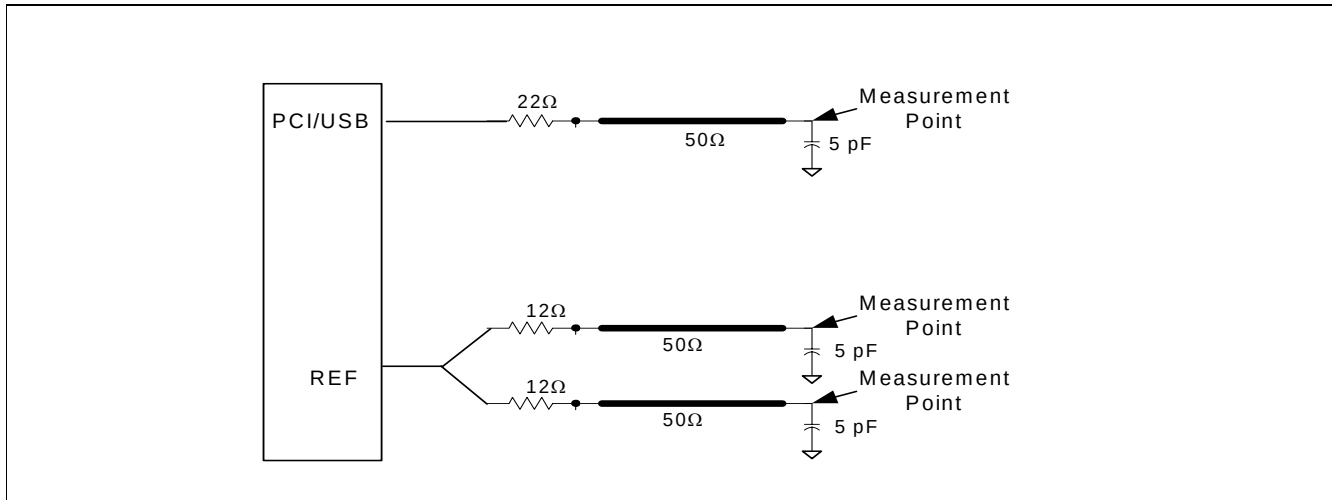
Figure 12. Single-ended Load Configuration.
