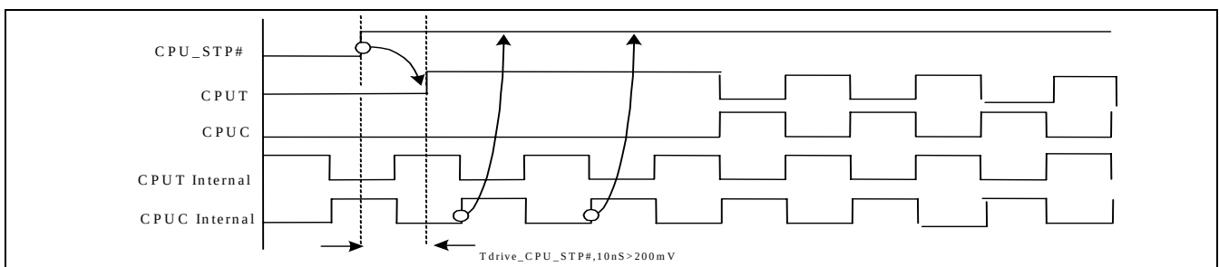
Figure 6. CPU_STP# Deassertion
