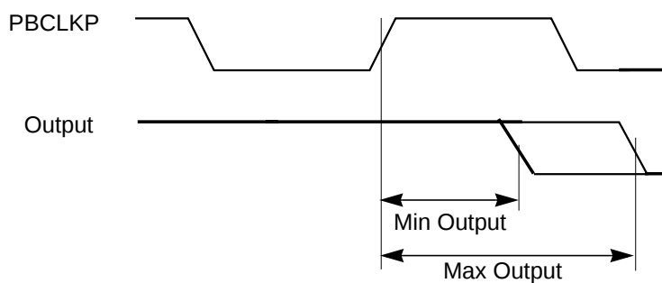
Figure 6 Output Timing with Respect to PBCLKP
