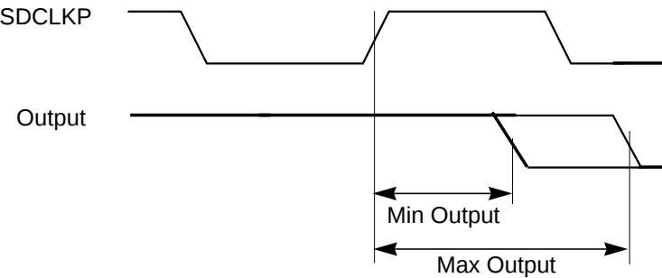
Figure 8 Output Timing with Respect to SDCLKP
