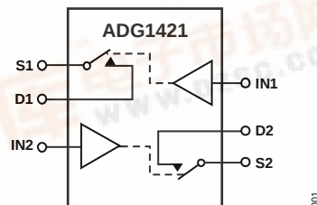
Figure 1. ADG1421 Functional Block Diagram
