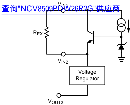
Figure 42. Power Shunt
