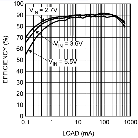
Efficiency vs. Output Current Auto Mode, V_{OUT2} = 1.5V
