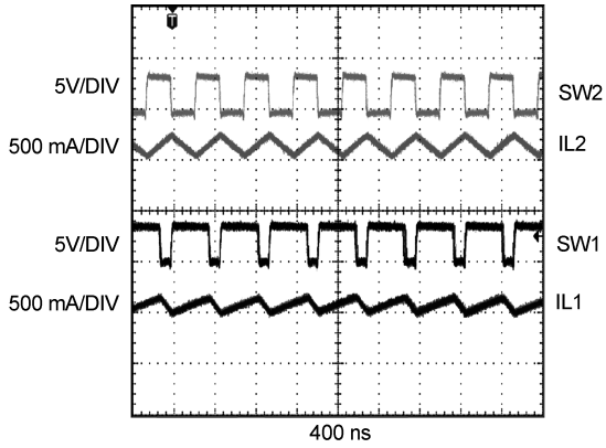
Typical Operation Waveform 查询LM3370SDX-30V1V供应商 V_{IN} = 3.6V , V_{OUT1} = 3.5V , V_{OUT2} = 1.5V , Load = 600 mA Each
