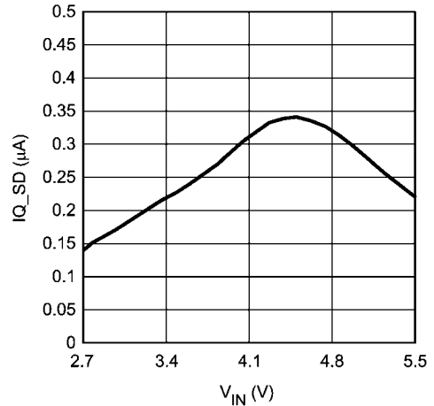
IQ_SD (EN1 = EN2 = 0V)
