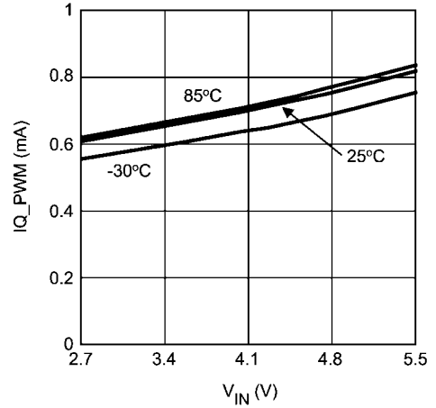
IQ_PWM (Non Switching) Both Channels
