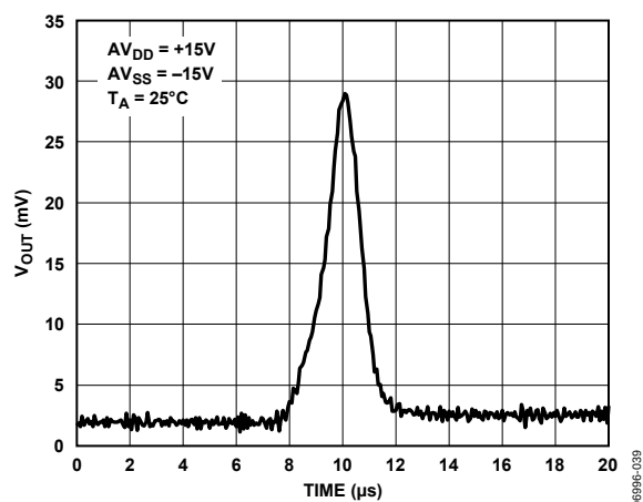
Figure 41. V OUT vs. Time on Power-Up
