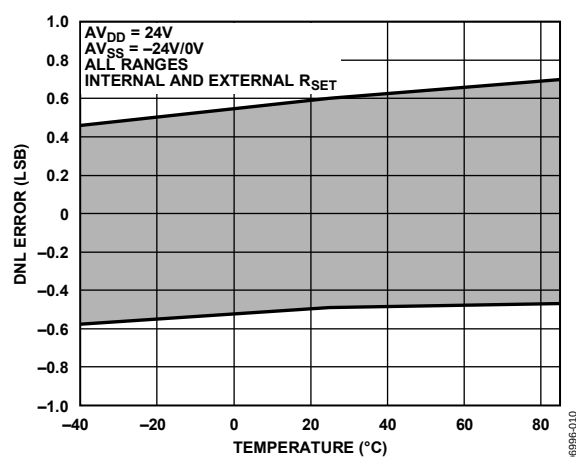
Figure 47. Differential Nonlinearity vs. Temperature
