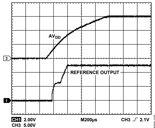
Figure 11. REFOUT Turn-on Transient
