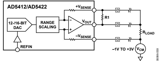
Figure 65. Voltage Output
