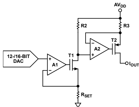
Figure 64. Voltage-to-Current Conversion Circuitry
