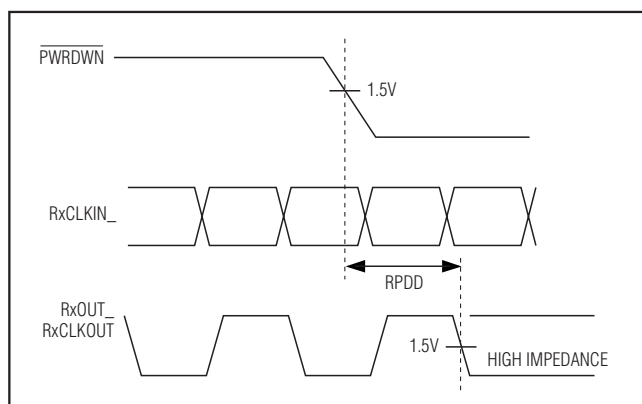
Figure 8. Power-Down Delay
