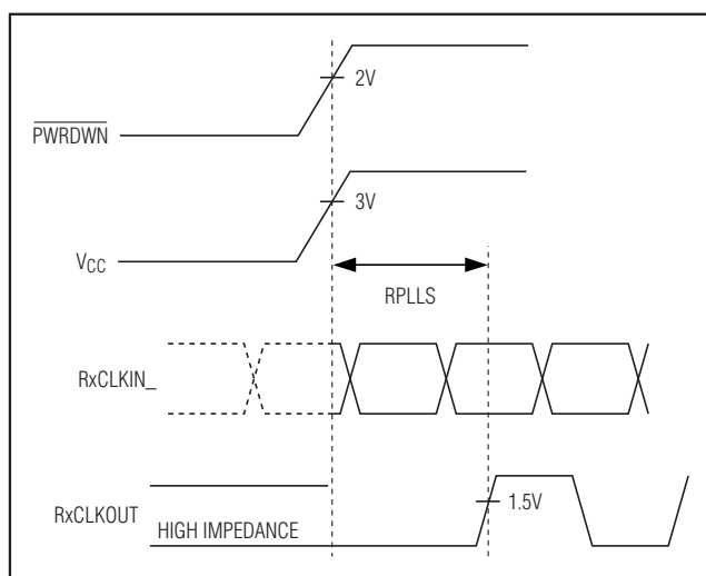
Figure 7. Phase-Locked-Loop Set Time
