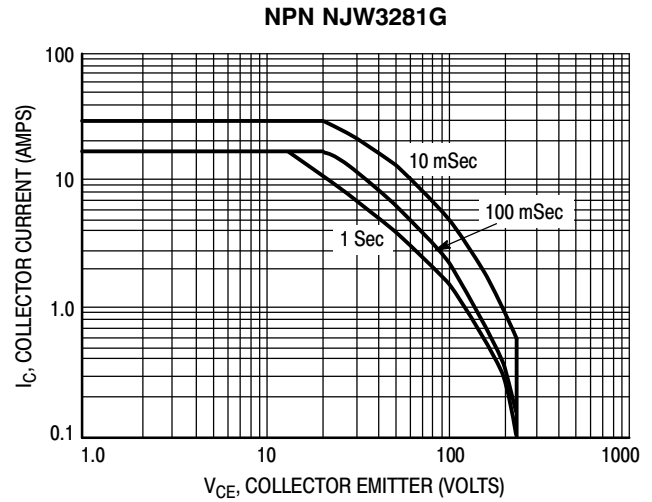
Figure 18. Active Region Safe Operating Area
